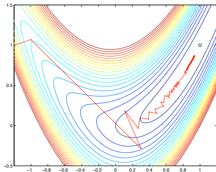
Steepest descent
