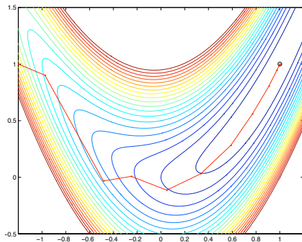
Newton's method
